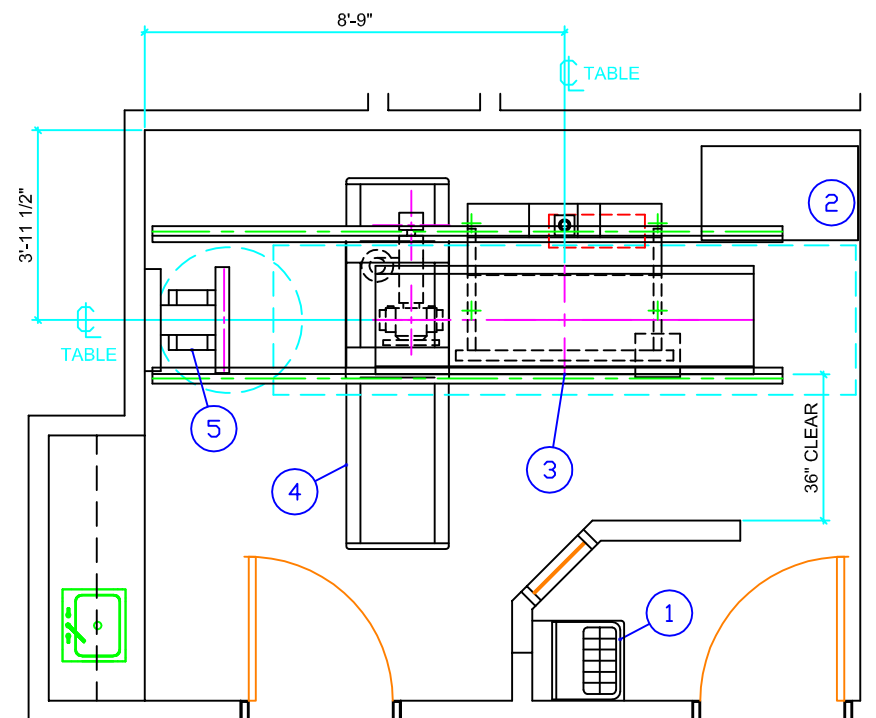
TYPICAL ROOM AND EQUIPMENT LAYOUT
