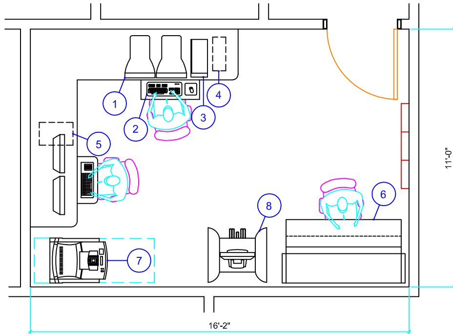
TYPICAL ROOM AND EQUIPMENT LAYOUT
