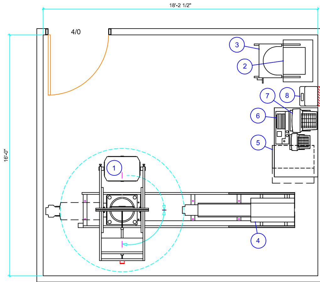
TYPICAL ROOM AND EQUIPMENT LAYOUT (DASHED LINES DEPICT TABLE TOP TRAVEL AND SFD CLEARANCE.)
